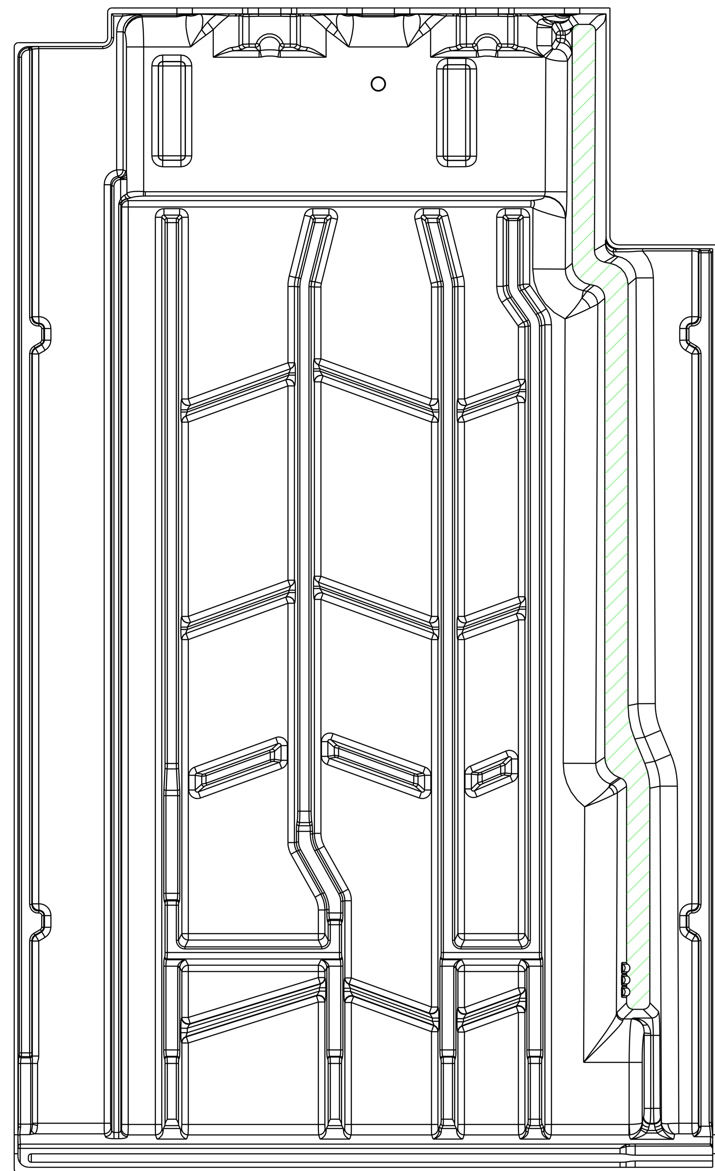
SECTION C-C
