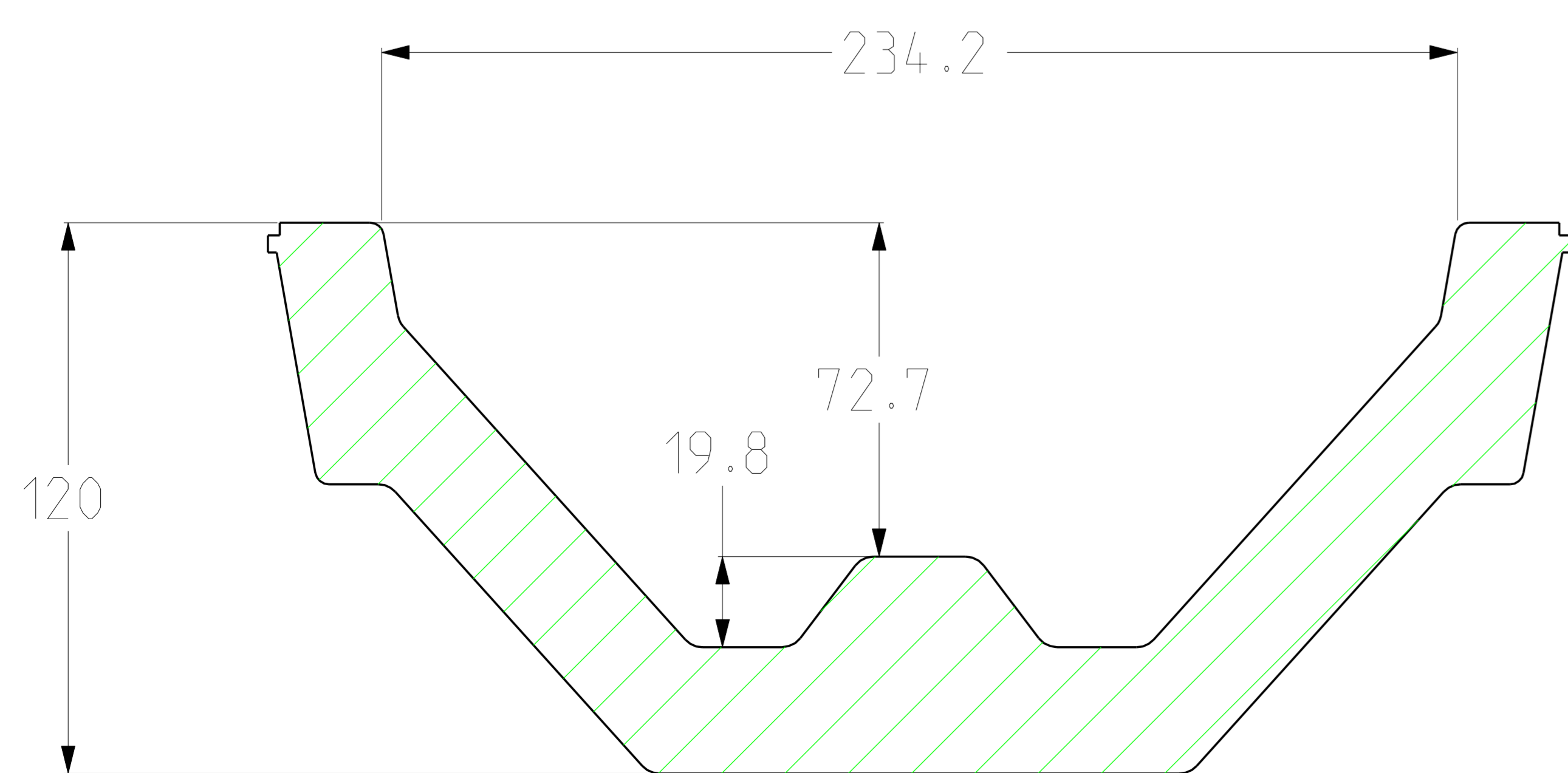
SECTION B-B
